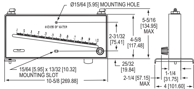
Inclined manometer
